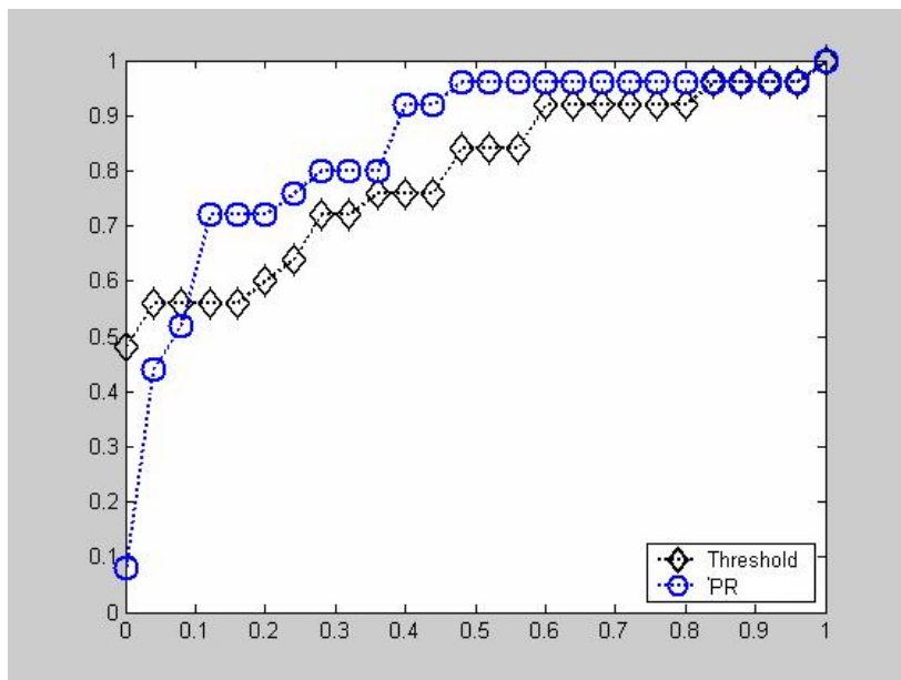
Figure 4.4: ROC curves for the PR score and TH density measures with an area under the curve of 0.82 and 0.76 respectively
